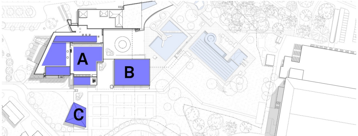
Situationsplan Photovoltaikanlage
